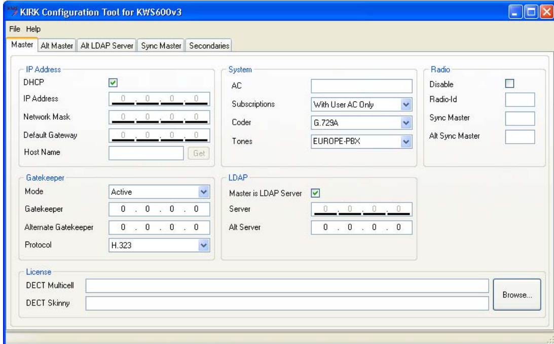
Figure 31 KIRK Configuration Tool startup window
